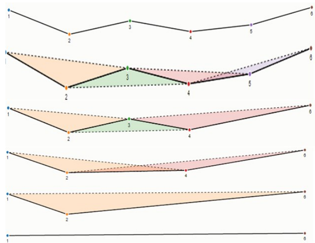
Fig. 1. Curve approximation by Visvalingam-Whyatt algorithm
