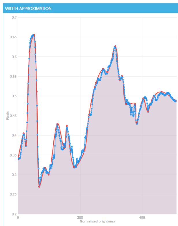
Fig. 4. Brightness function approximation (width) by Visvalingam-Whyatt algorithm (tolerance = 0.75)
