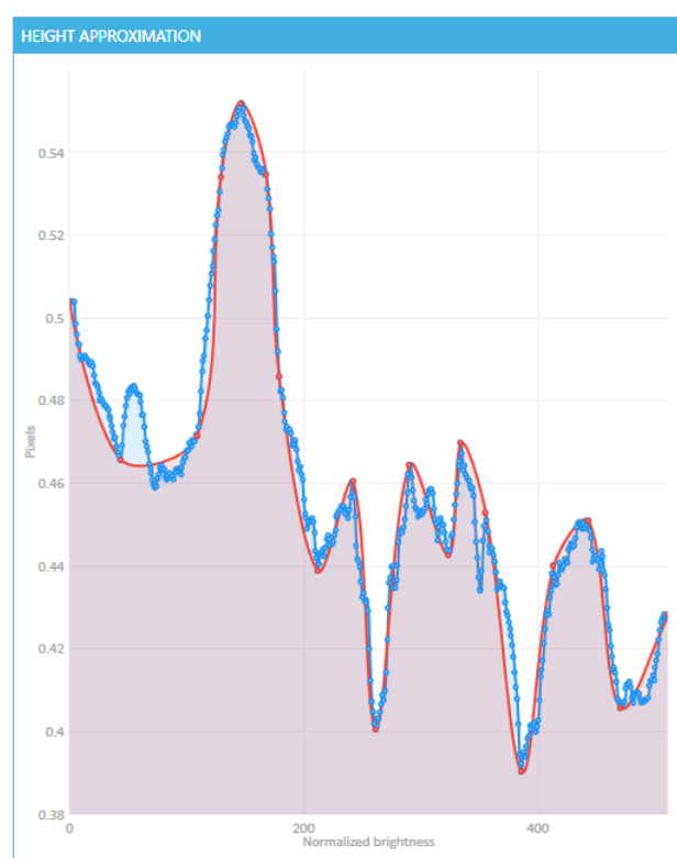
Fig. 5. Brightness function approximation (height) by Visvalingam-Whyatt algorithm (tolerance = 0.75)
