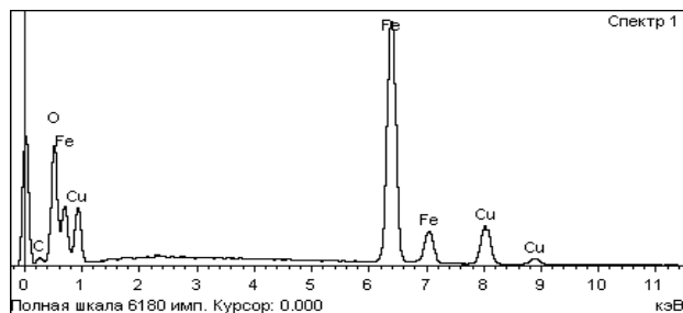
Fig. 1. Spectrum of the Fe-Cu bimetal surface
