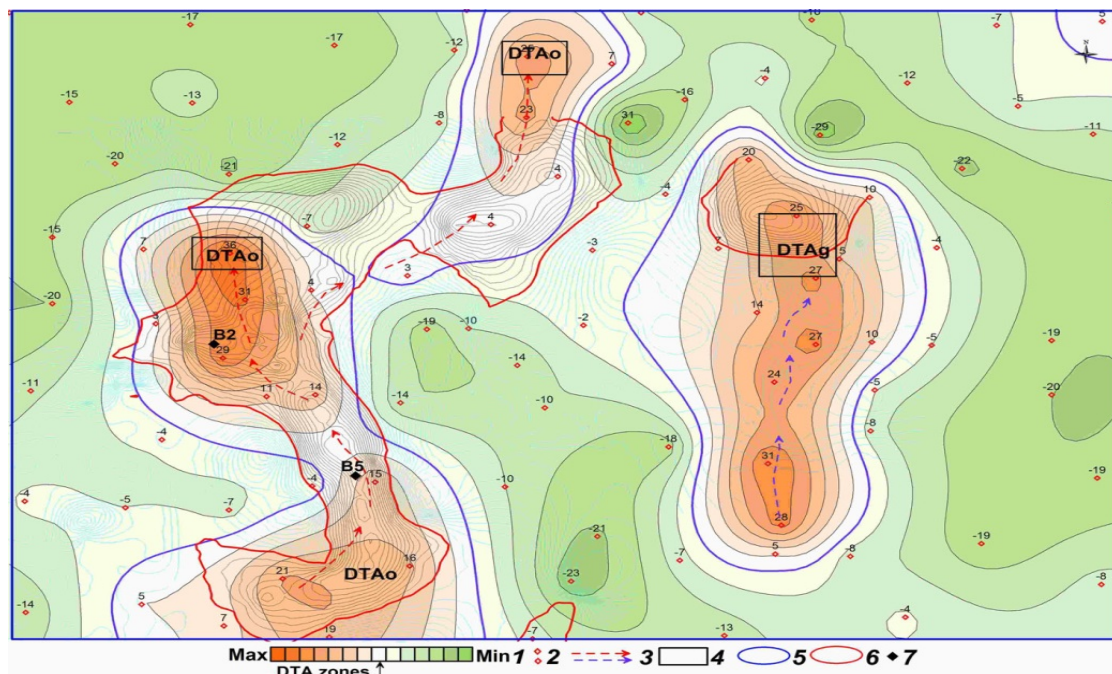
Figure 1 Schematic map of the results of the satellite image frequency-resonance processing of search area in the Black Sea region. 1 – scale of the anomalous response intensity; 2 – points of the anomalous response determining; 3 – projected directions of HC migration; 4 – areas recommended for detailed study and drilling; 5 – outlines of the anomalies according to satellite image processing; 6 – outlines of the anomalies according to the ground-based geoelectric survey by FSPEF method; 7 – points of VERS sounding
